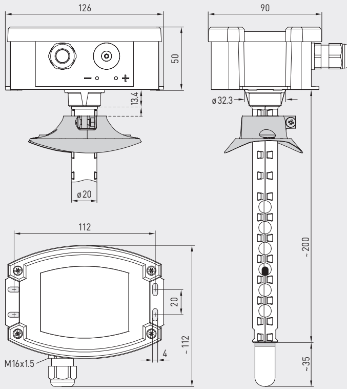
Dimensional drawing [mm]
