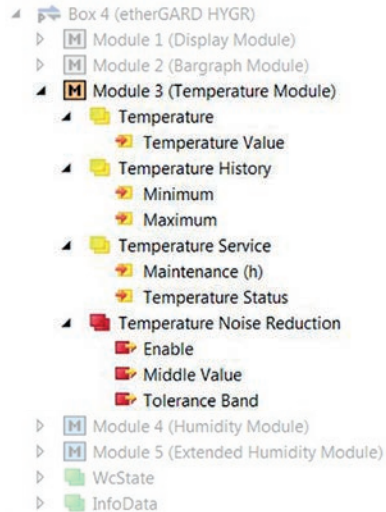
Fig. 2 Process data objects (PDO) of the temperature module
