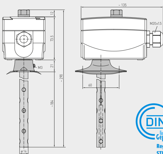
Dimensional drawing Safety temperature limiter
