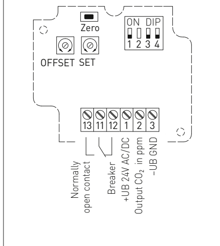
Connecting diagram KCO2-W
