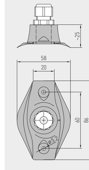
Dimensional drawing KRD-04
