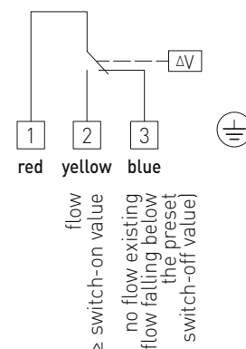
Connecting diagram
