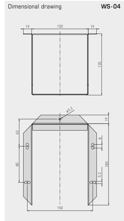
WS-04 Weather and sun protection hood
