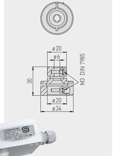
Dimensional drawing TH-ADAPTER-HW
