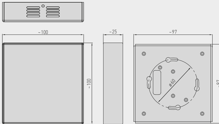
Dimensional drawing
