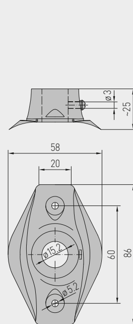
Dimensional drawing MF-15-K
