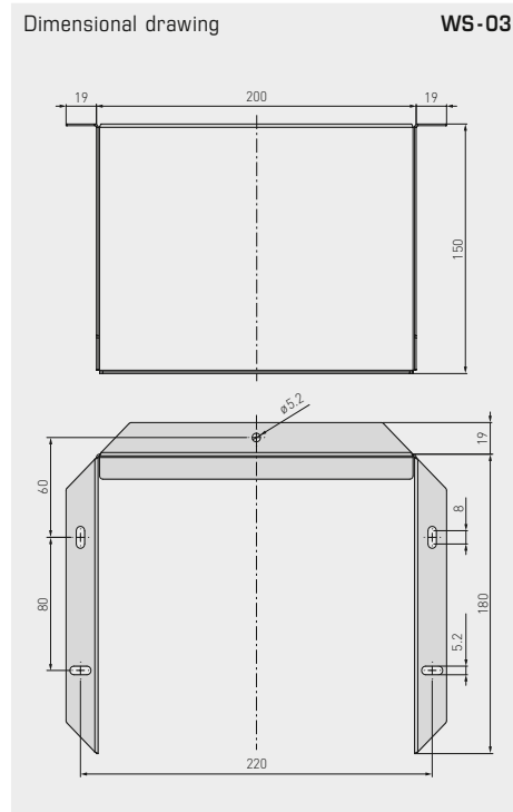
WS-03 Weather and sun protection hood
