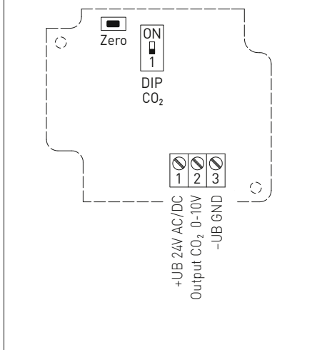
Connecting diagram KCO2-SD
