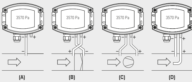
Mounting diagram
