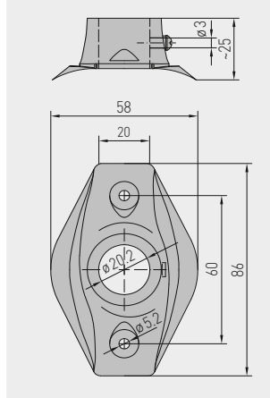
Dimensional drawing MF-20-K
