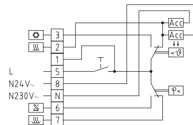
Connecting diagram
